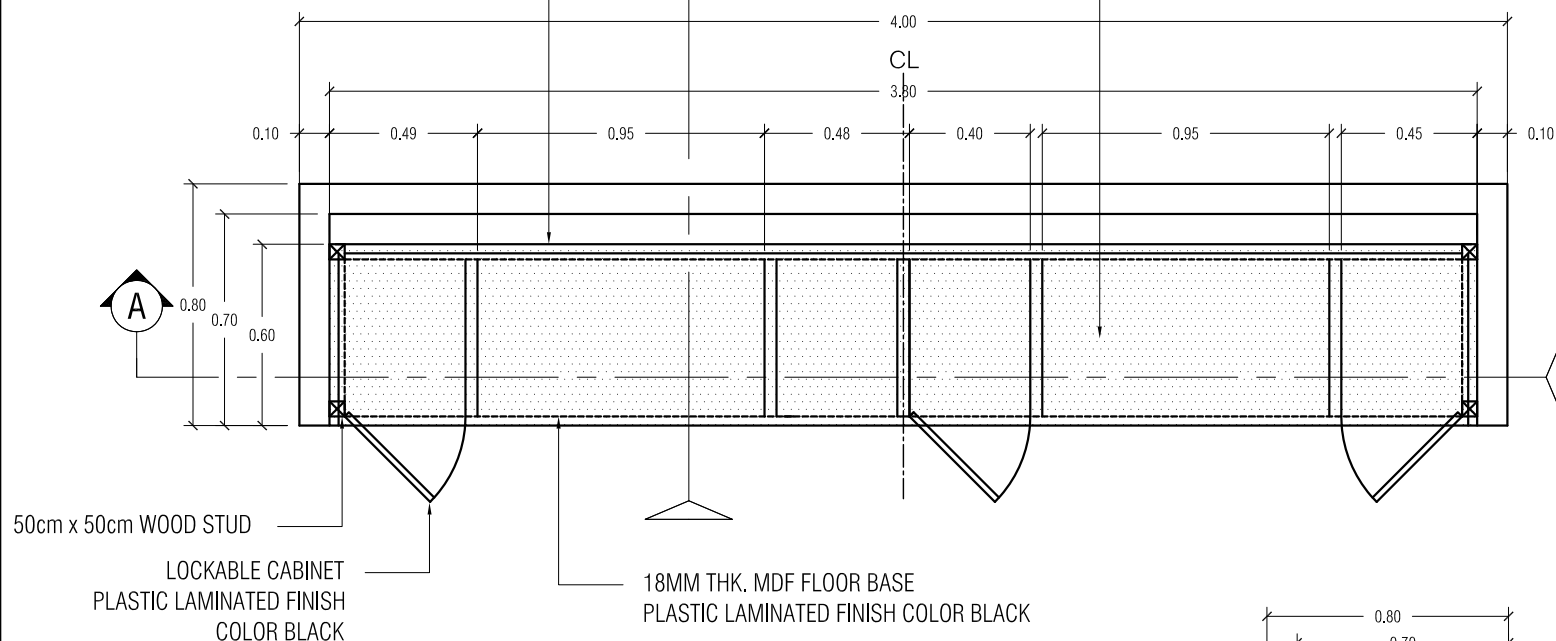
A-16 01 1 SET RECEPTION COUNTER PLAN & DETAILS SCALE 1:50 M
