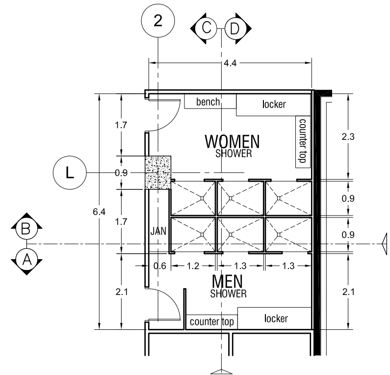
A-12 01 MEN WOMEN SHOWER ROOM SCALE 1:100M
