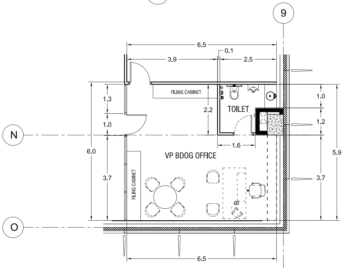
A-05 02 BDOG OFFICE SCALE 1:100M
