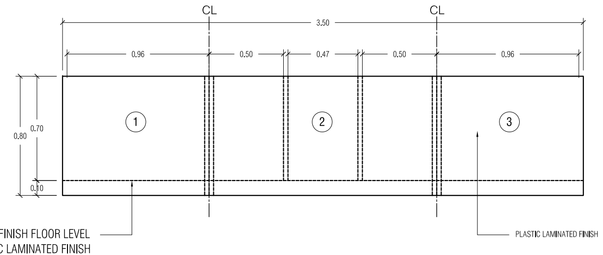
A-14 03 BACK VIEW SCALE 1:50 M
