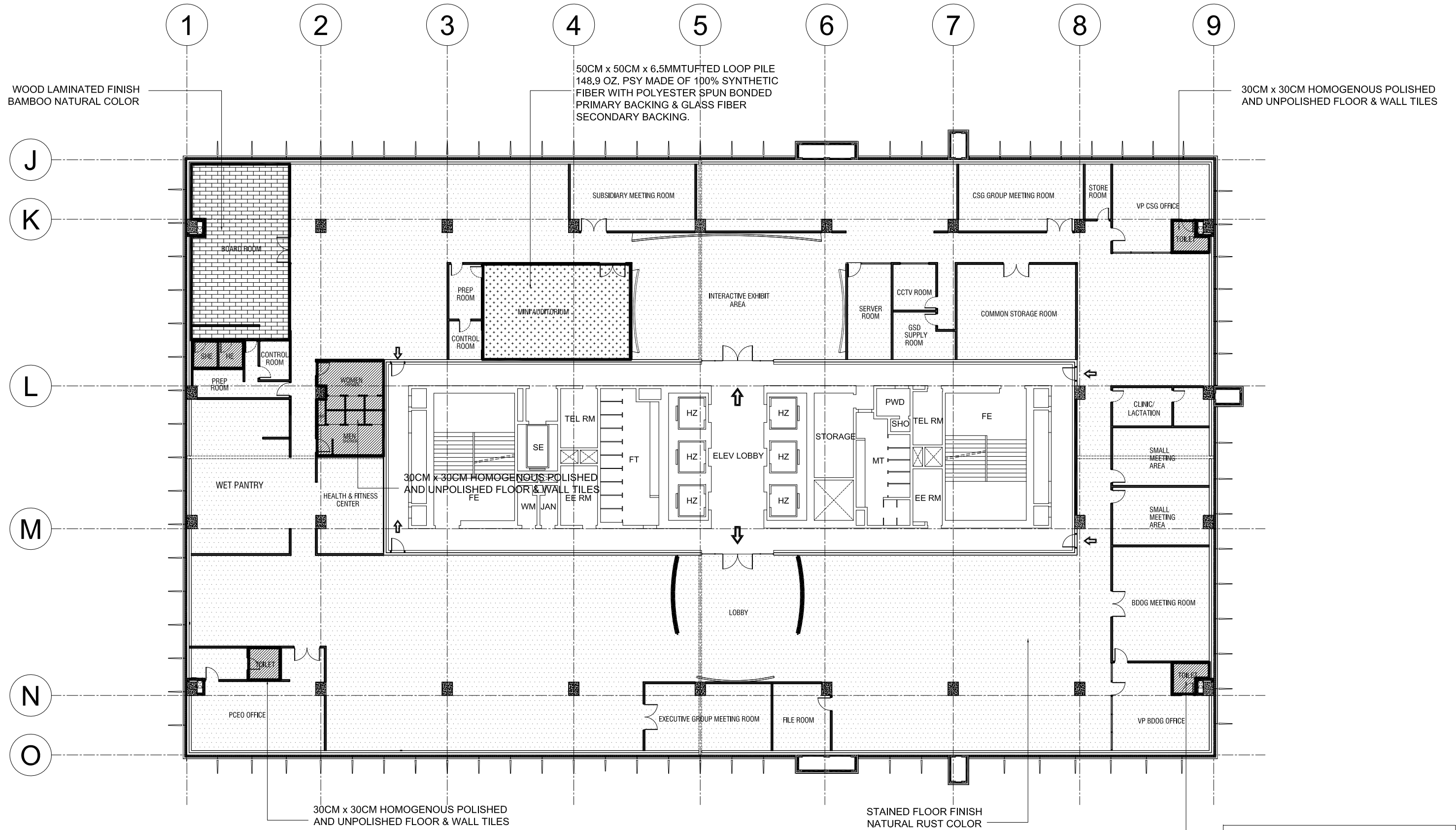
FLOOR FINISHES PLAN
