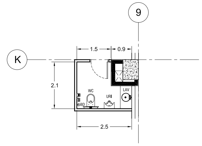
A11 4 CSG TOILET SCALE 1:100M
