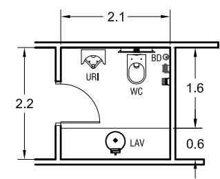
A11 2 PCEO TOILET SCALE 1:100M
