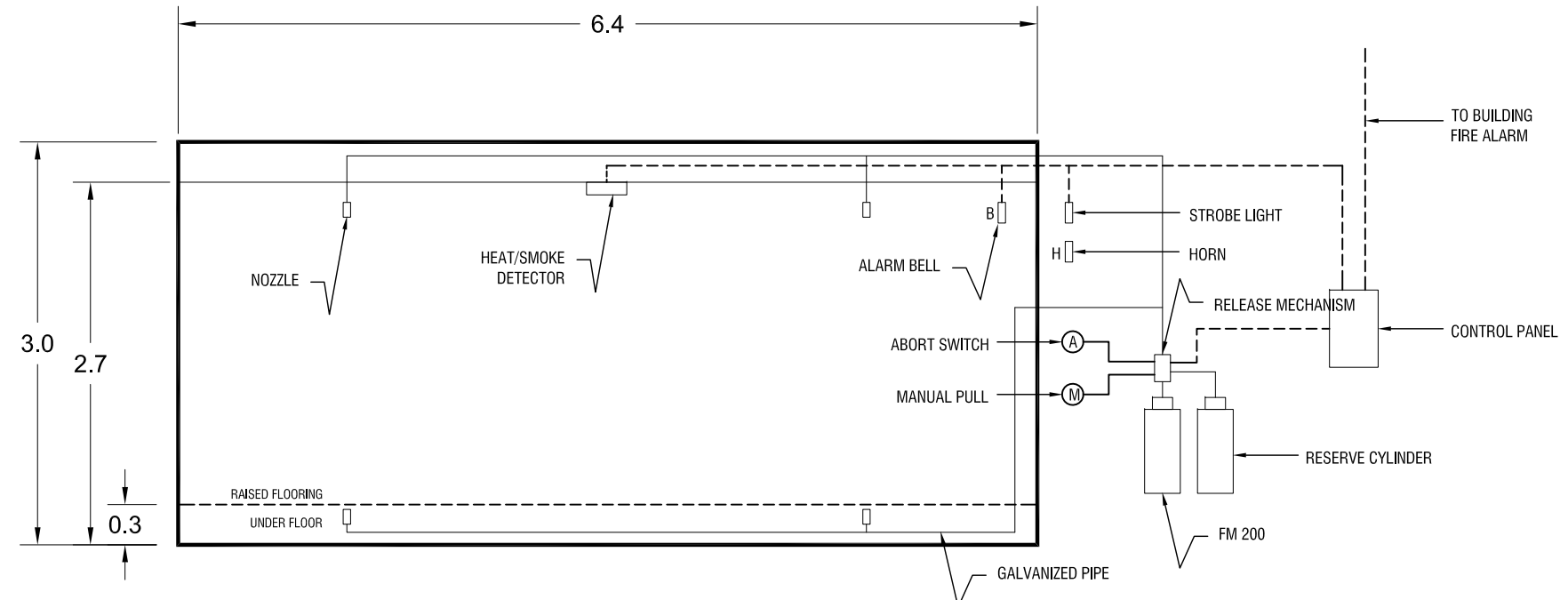
M3 2 FM- 200 SCHEMATIC DIAGRAM SCALE 1:50M
