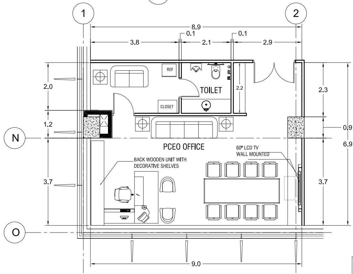
A-05 02 PCEO OFFICE SCALE 1:100M
