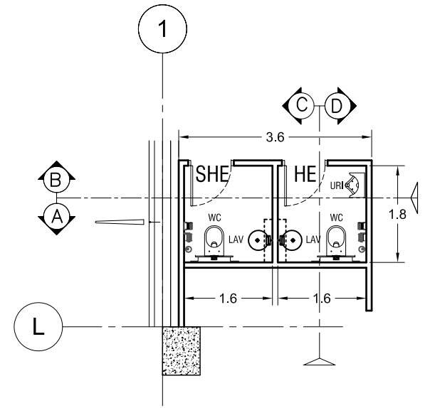
A11 1 BOARDROOM TOILET SCALE 1:100M
