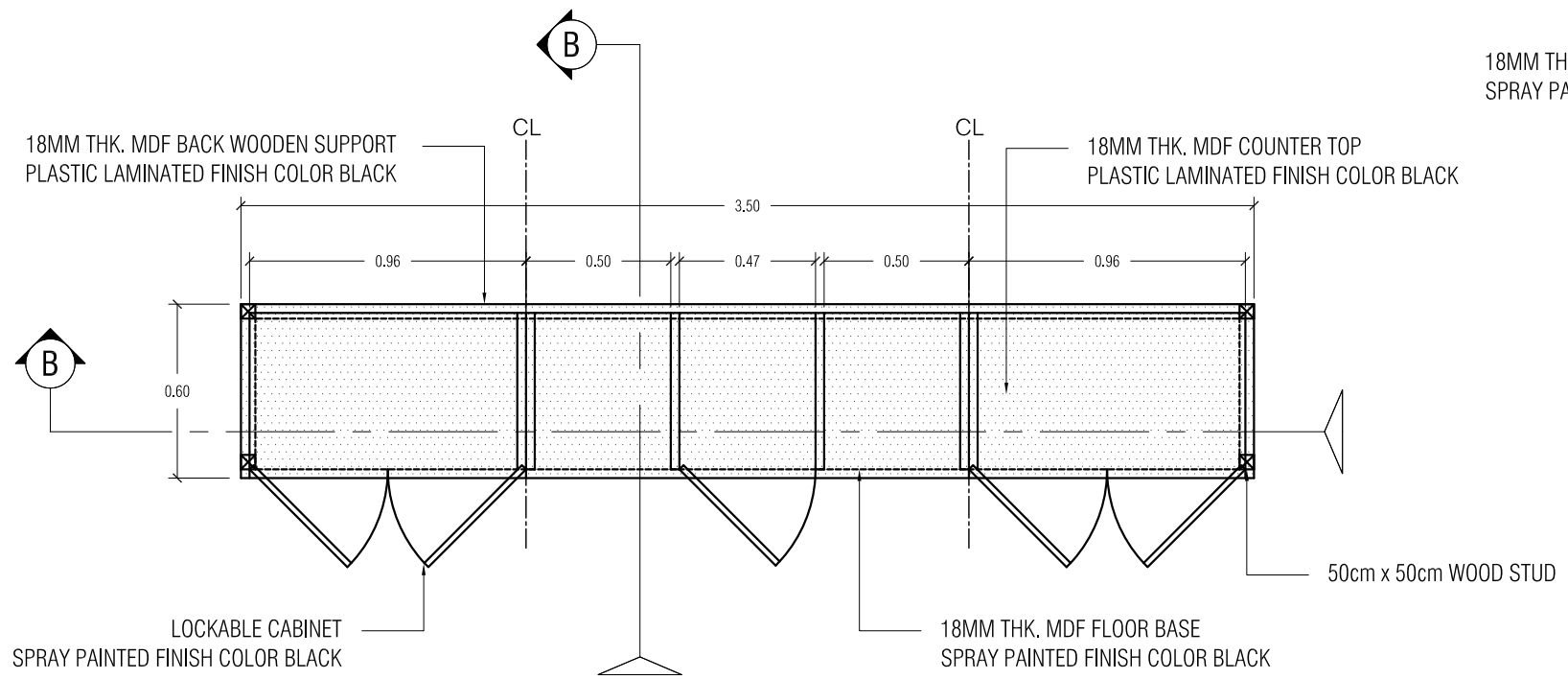
A-14 01 4 SETS CABINET 1 PLAN & DETAILS SCALE 1:50 M
