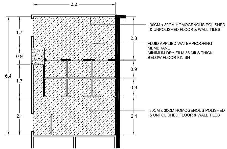
29 M2 A-12 02 WATER PROOFING PLAN SHOWER ROOM SCALE 1:100M
