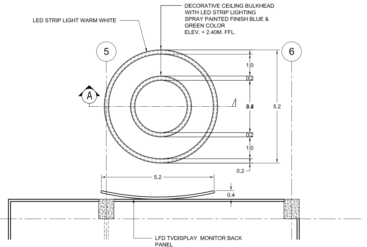
A17 2 SCALE 1:100M RECEPTION AREA DECORATIVE CEILING
