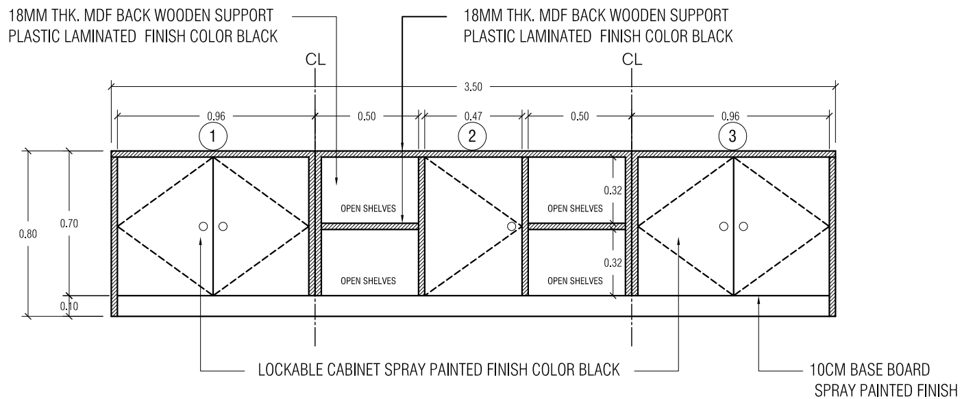
A-14 02 FRONT VIEW SCALE 1:50 M
