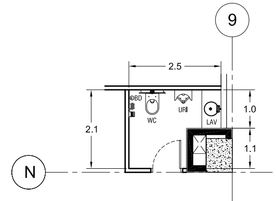
A11 3 BDOG TOILET SCALE 1:100M
