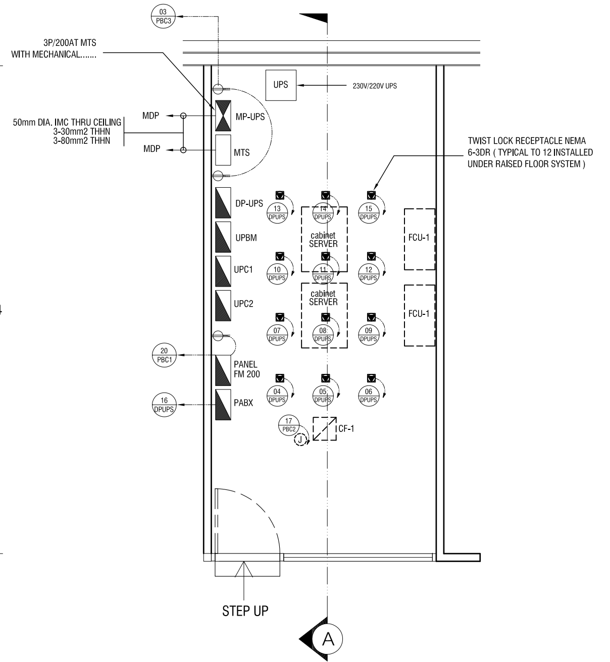
M2 1 SERVER ROOM ELECTRICAL BLOW UP PLAN SCALE 1:50M
