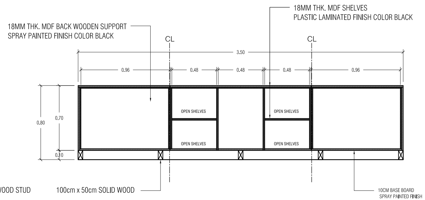
A-14 03 BACK VIEW SCALE 1:50 M
