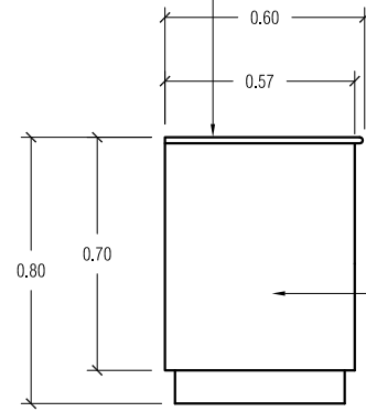
A-15 03 TYP. SIDE VIEW SCALE 1:50 M
