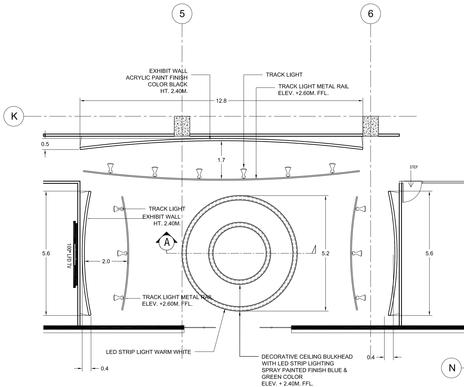
A17 1 SCALE 1:100M INTERACTIVE EXHIBIT AREA DECORATIVE CEILING
