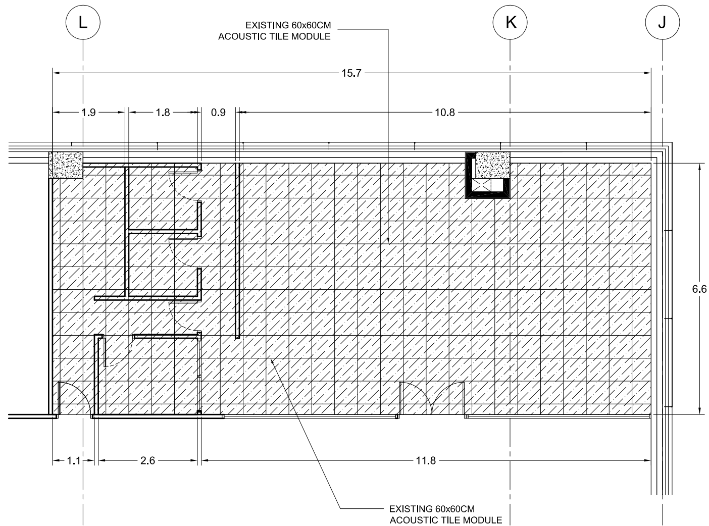
A-07 02 BOARD ROOM CEILING PLAN SCALE 1:100M
