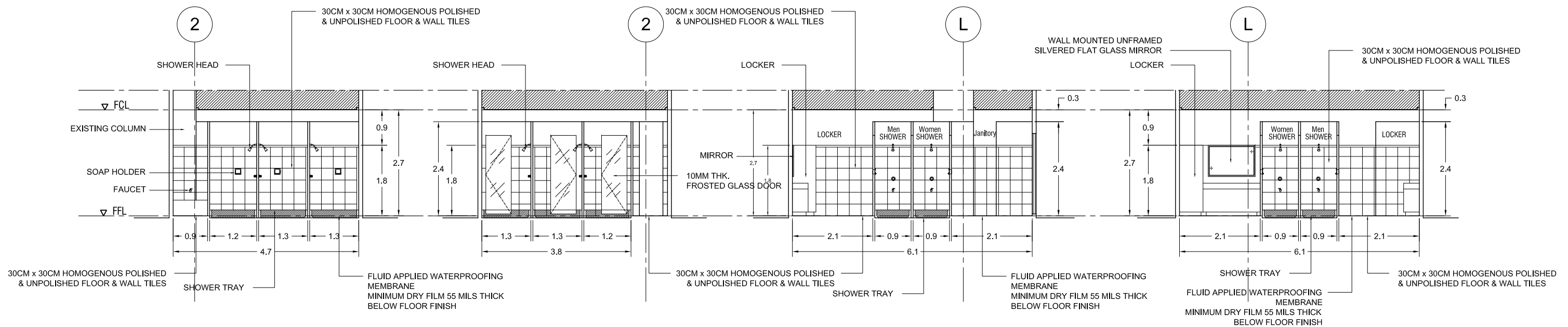
A-12 03 MEN WOMEN SHOWER ROOM SECTION B-B SCALE 1:100M
