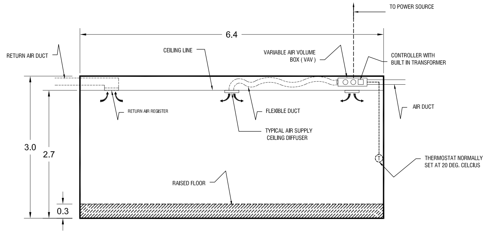
M3 1 SECTION A-A TYPICAL ROOM COOLING SYSTEM DIAGRAM SCALE 1:50M
