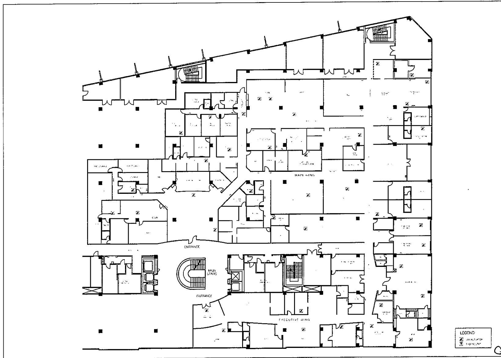
LOCATION OF VAV AND THERMOSTAT
